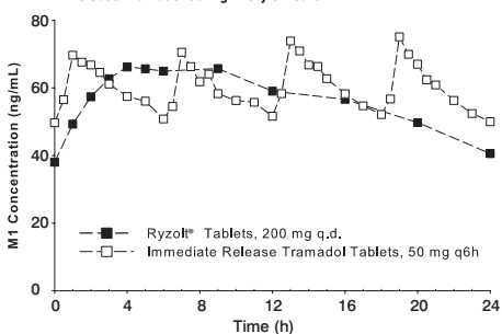
Figure 2. Mean M1 Plasma Concentrations at Steady State Following Five Days of Oral Administration of RYZOLT ® 200 mg Once Daily and Immediate-Release Tramadol 50 mg Every 6 Hours
