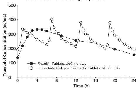
Figure 1. Mean Tramadol Plasma Concentrations at Steady State Following Five Days of Oral Administration of RYZOLT ® 200 mg Once Daily and Immediate-Release Tramadol 50 mg Every 6 Hours.
